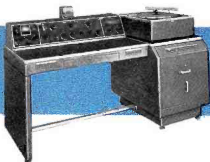
1939. This custom-built audio console for WOR was the first commercial type meeting all requirements for FM use. It provided circuits and equipment to meet specific operating conditions. The tailored metal desks mounted amplifiers, control and switching equipment and turntable units—all within easy reach of the operator.
